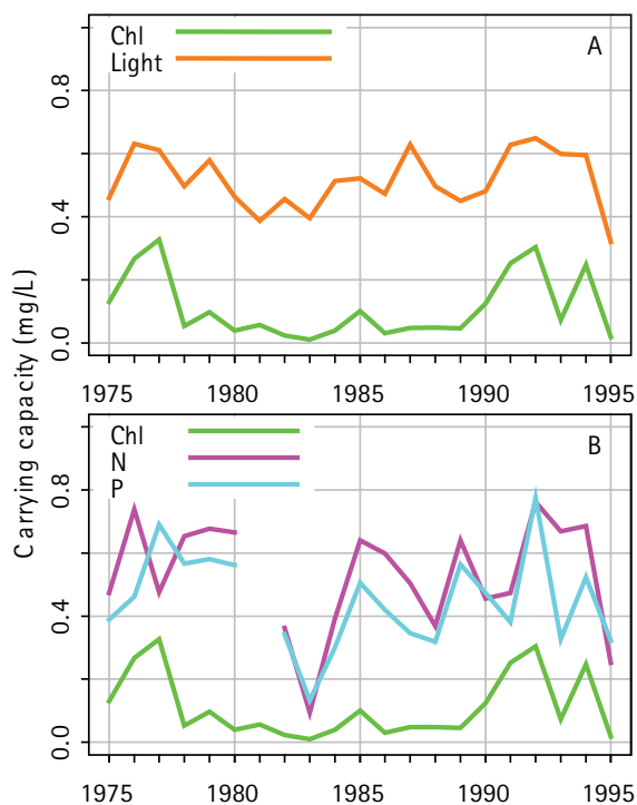
Figure 5. Estimated carrying capacities of available resources at Mossdale for phytoplankton, compared with actual chlorophyll a values. (A) Light carrying capacity. (B) Nitrogen and phosphorus carrying capacities.
