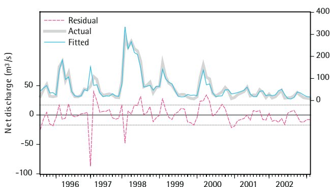
Figure 13. Fitted values and actual observations of net discharge into the Ship Channel. Fitted values are based on the model described by Equation 8. Horizontal dashed lines , standard error of residuals.
