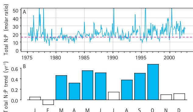
Figure 6. (A) Molar ratio of total nitrogen to phosphorus at Vernalis. Dashed line , ratio = 16, characteristic of phytoplankton. (B) Long-term (Theil) trends by month for the molar ratio of total nitrogen to phosphorus at Vernalis, 1975-2002. Shading , significantly different from zero ( P < 0.05 ), according to the Kendall-tau test.
