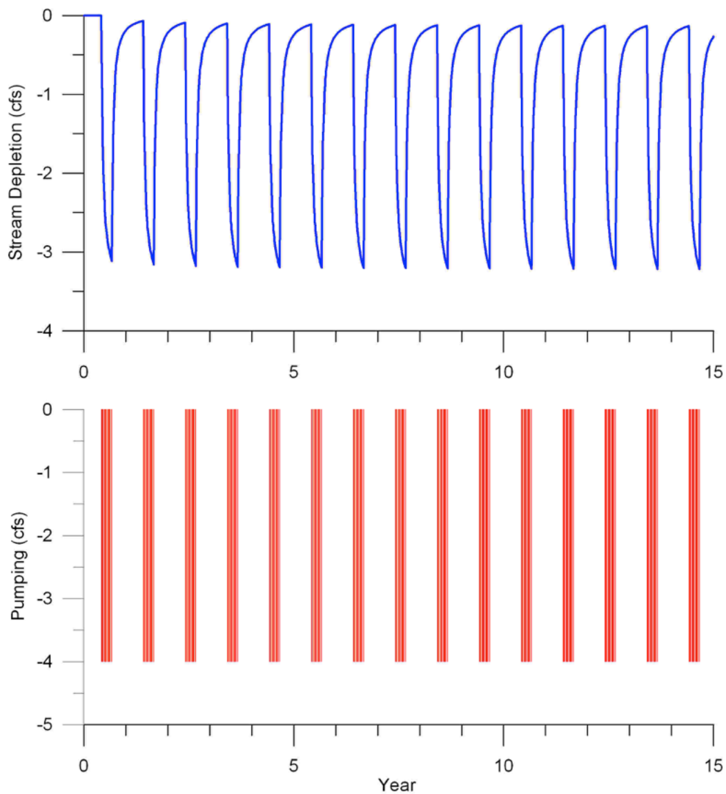
Figure 1 Reduction in streamflow (stream depletion, upper graph) created by a well located less than one-quarter mile from a stream pumping at a rate of 4.0 cfs (0.11 m 3 s) for 3 months annually (lower plot)
