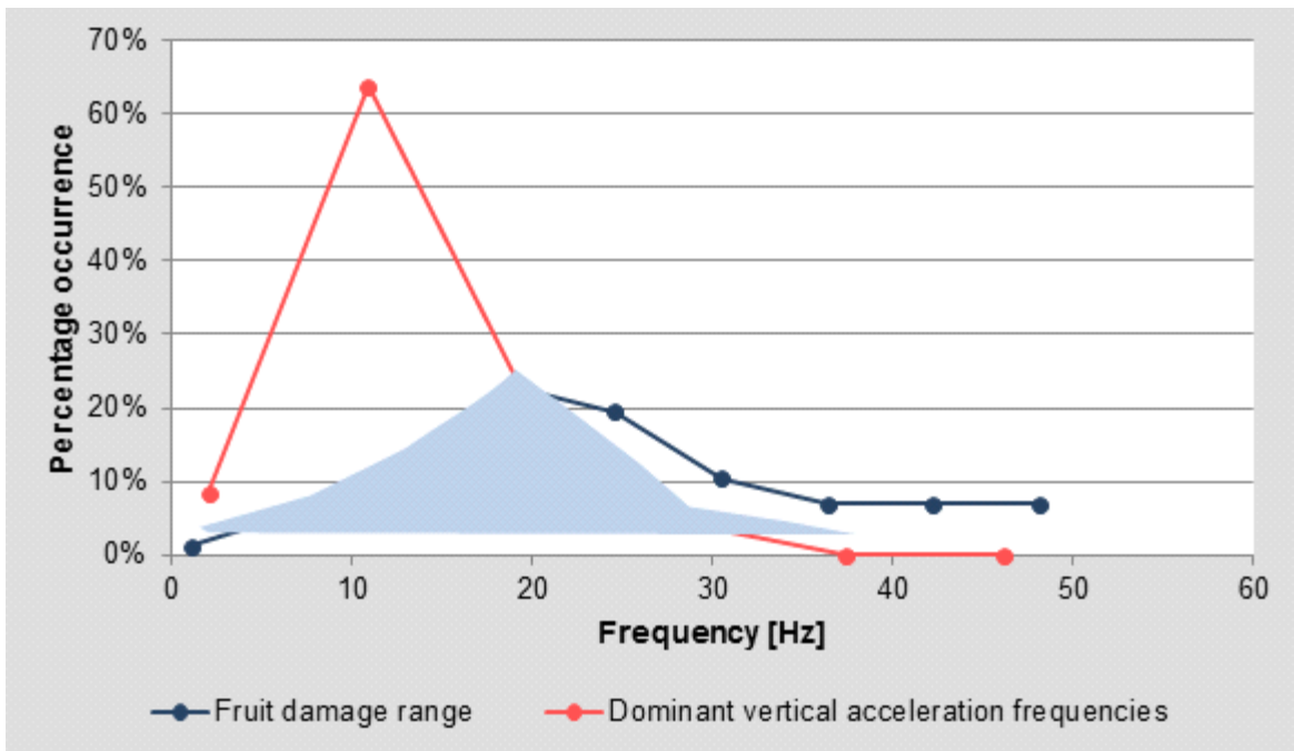
Figure 5.12: Comparison between dominant frequencies experienced by fruit cargo and the vibration range that results in damage.
