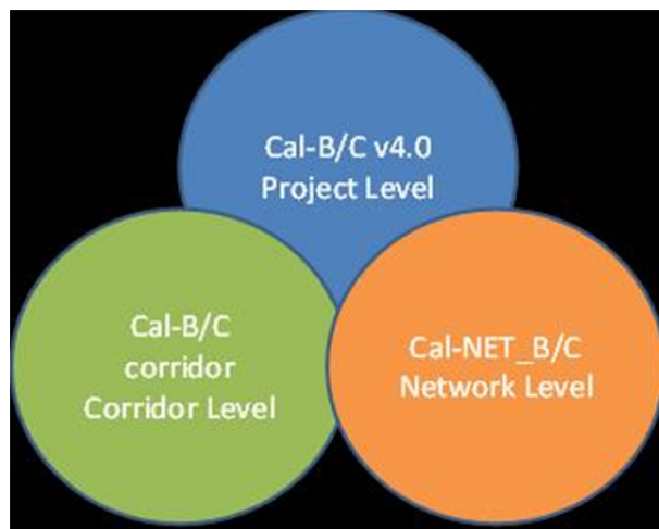
Figure 5.7: Cal-B/C framework.
