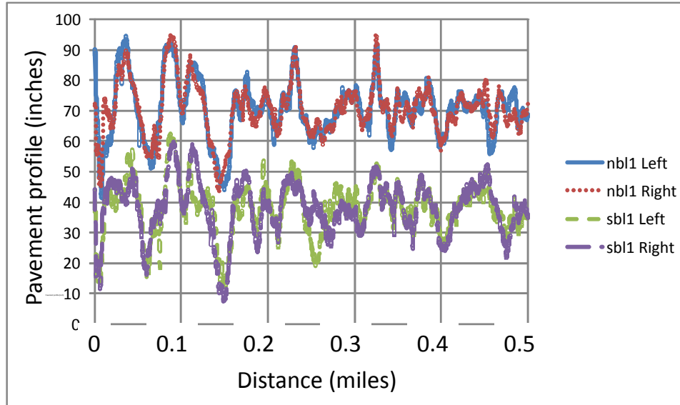
Figure 3.1: Example of four typical road profiles.
