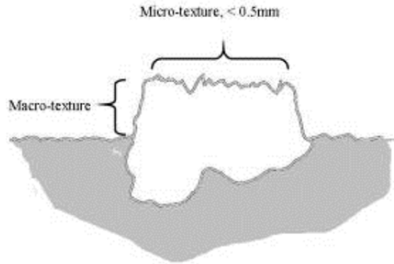
Figure 3.2: Definition of macrotexture and microtexture of pavement surfacing aggregate (6).
