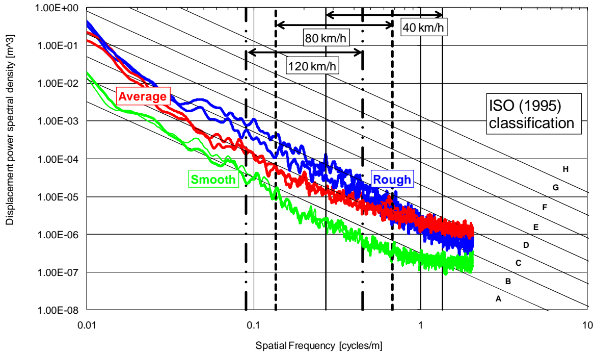
Figure 3.3: Displacement power spectral densities (DPSDs) on ISO classification for three different pavements.
