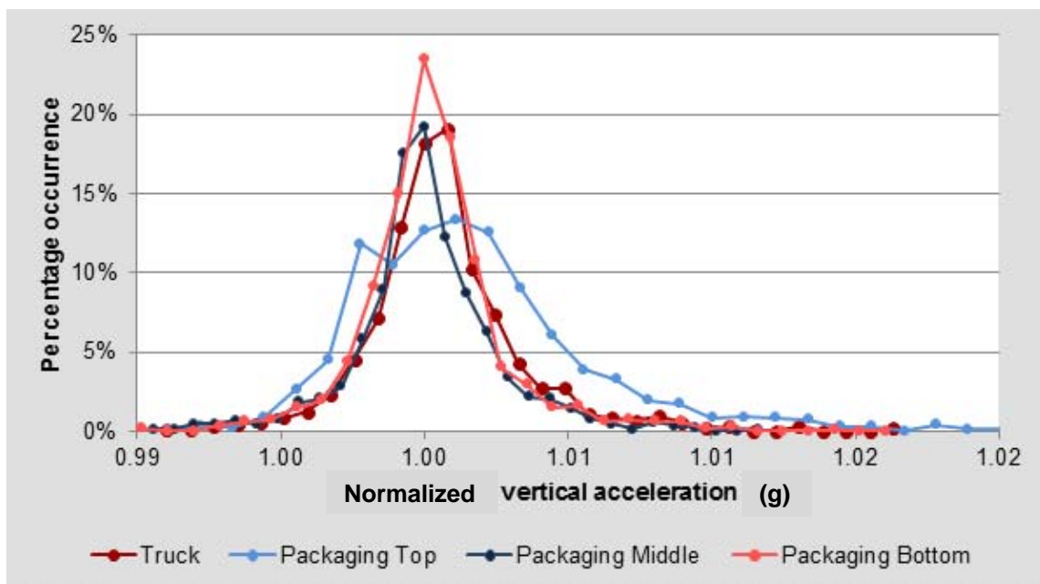
Figure 5.13: Normalized distributions of the vertical accelerations experienced within pallets at various packing levels at the front of the truck.
